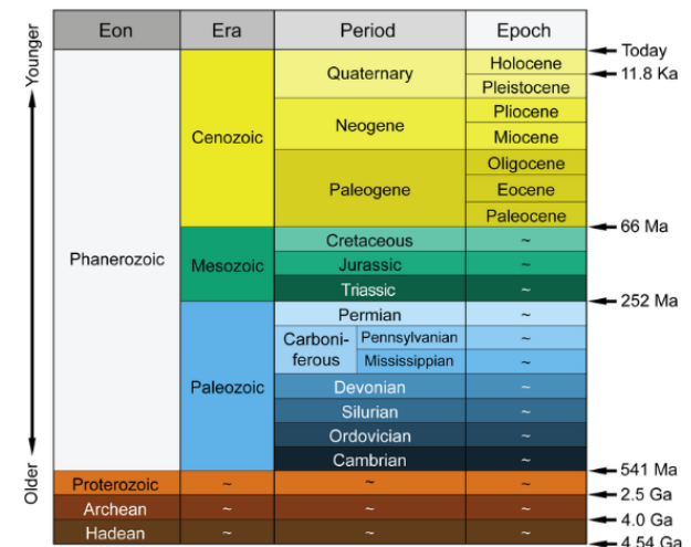
Geologic Time Scale. Credit: PRI's Earth@Home Project
